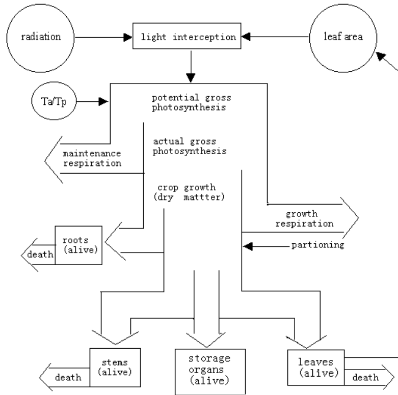
Figure 3. Crop growth processes ( T_a and T_p are actual and potential transpiration rate).
