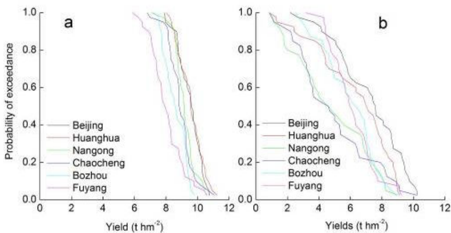
Figure 12. Cumulative distribution of (a) potential yield and (b) water-limited yield of summer maize for six locations in the North China Plain.
