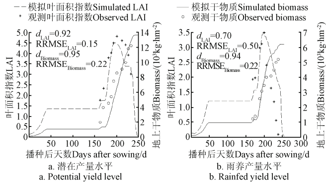
注: d_{LAI} 和 RRMSE_{LAI} 分别为叶面积指数的一致性指数和相对均方根误差, d_{Biomass} 和 RRMSE_{Biomass} 分别为地上干物质的一致性指数和相对均方根误差。 Note: d_{LAI} and RRMSE_{LAI} represent the index of agreement and relative root mean square error of LAI, d_{Biomass} and RRMSE_{Biomass} represent the index of agreement and relative root mean square error of Biomass
