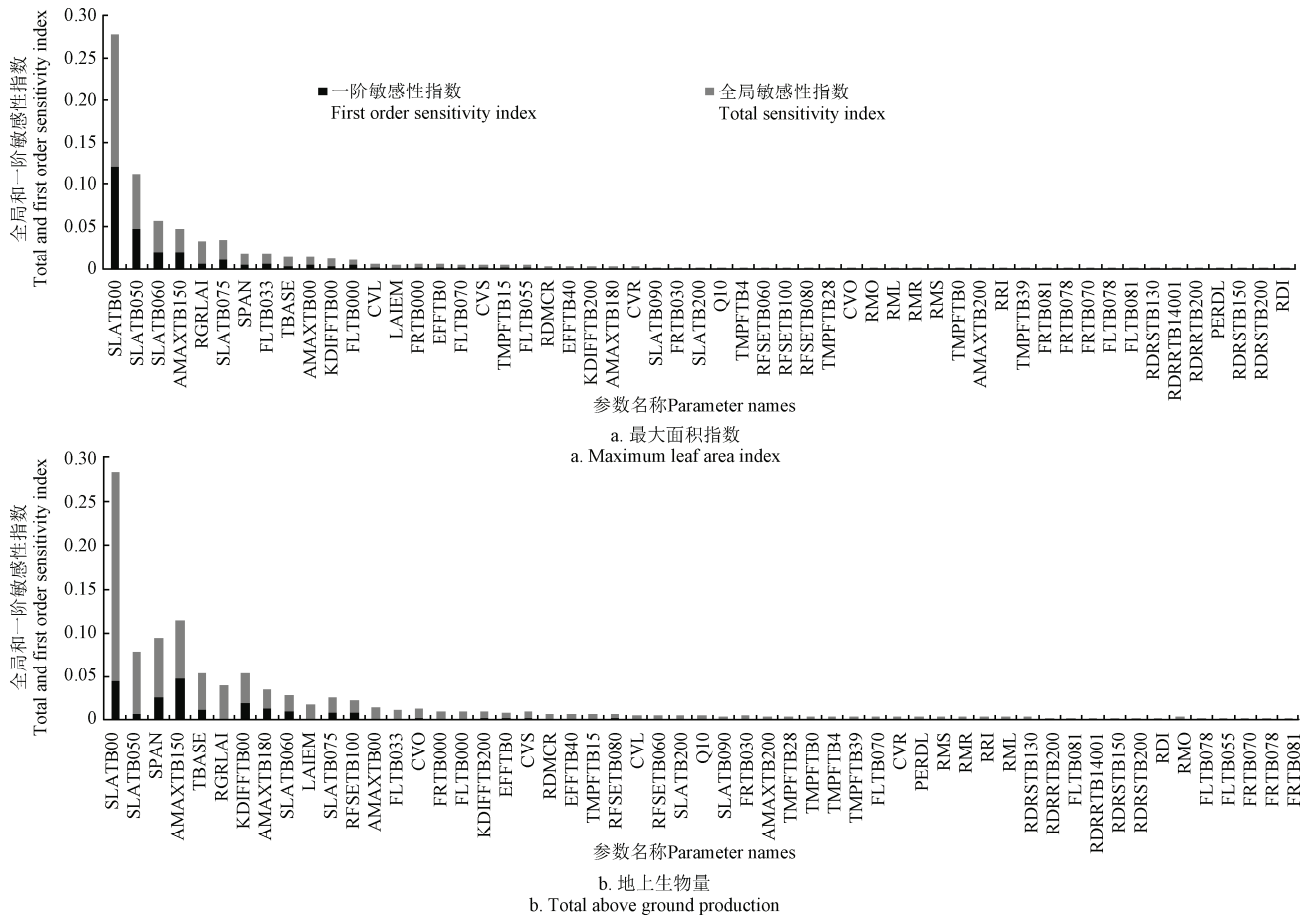
图 2 雨养产量水平下的扩展傅里叶幅度检验法的敏感性分析结果 Fig.2 Sensitivity results of extended Fourier amplitude sensitivity test in rain-fed yield level
