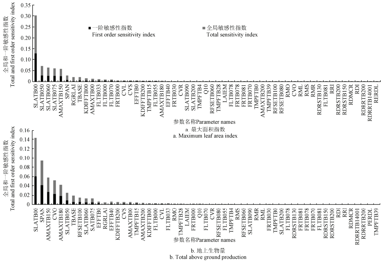
图 1 潜在产量水平下的扩展傅里叶幅度检验法的敏感性分析结果 Fig.1 Sensitivity results of extended Fourier amplitude sensitivity test in potential yield level
